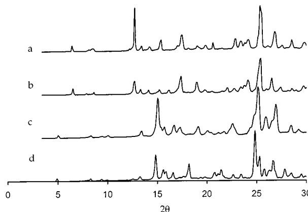
Figure 1. Powder diffraction patterns of complexes of Cephadrine with 2-hydroxyacetophenone (a) and methyl benzoate (b) (type A, C2 cavity) and with 2,2'-biphenol (c) and 2-phenylphenol (d) (C2 layers)
