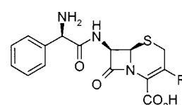
2 Cephalexin (R = CH 3 ) 3 Cefaclor (R = Cl)
